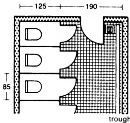
⑤ Doors opening outwards; with urinal trough
